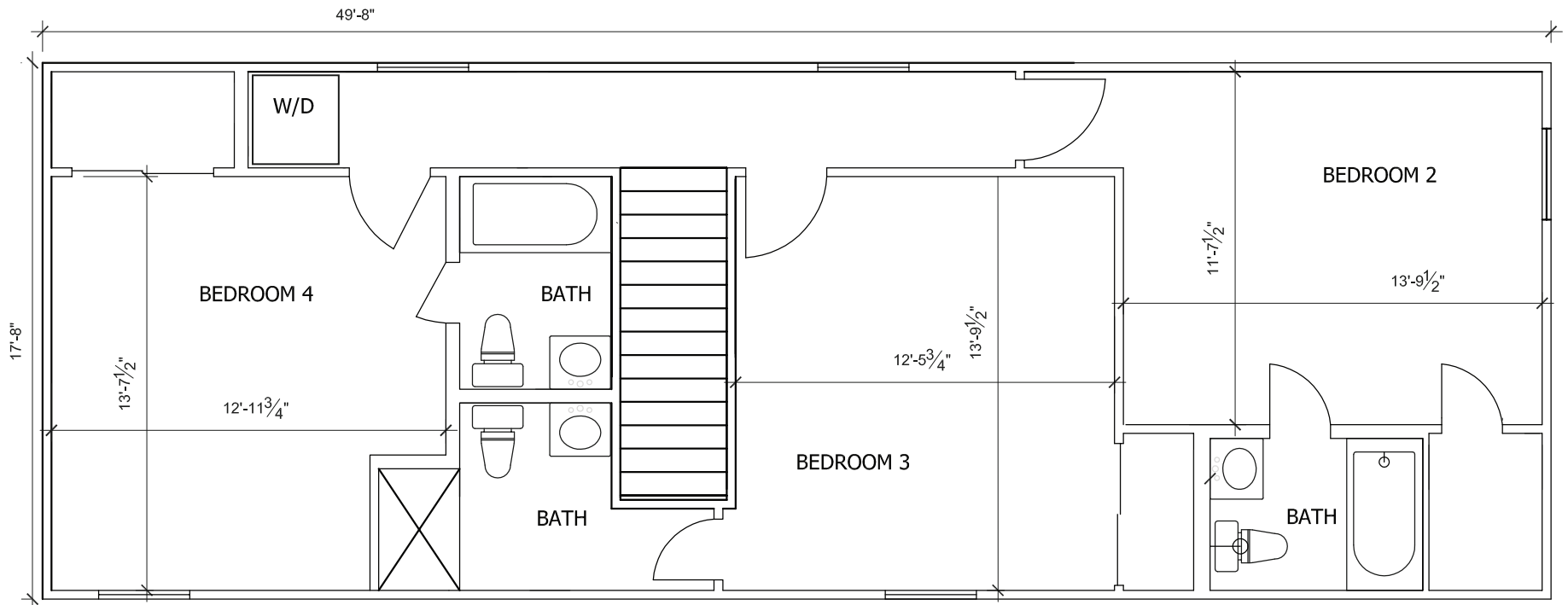
Second Floor
